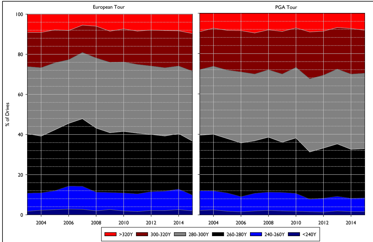
Figure 10. The distribution of drives on “measured” driving holes on the European and PGA tours 2003-2015.
