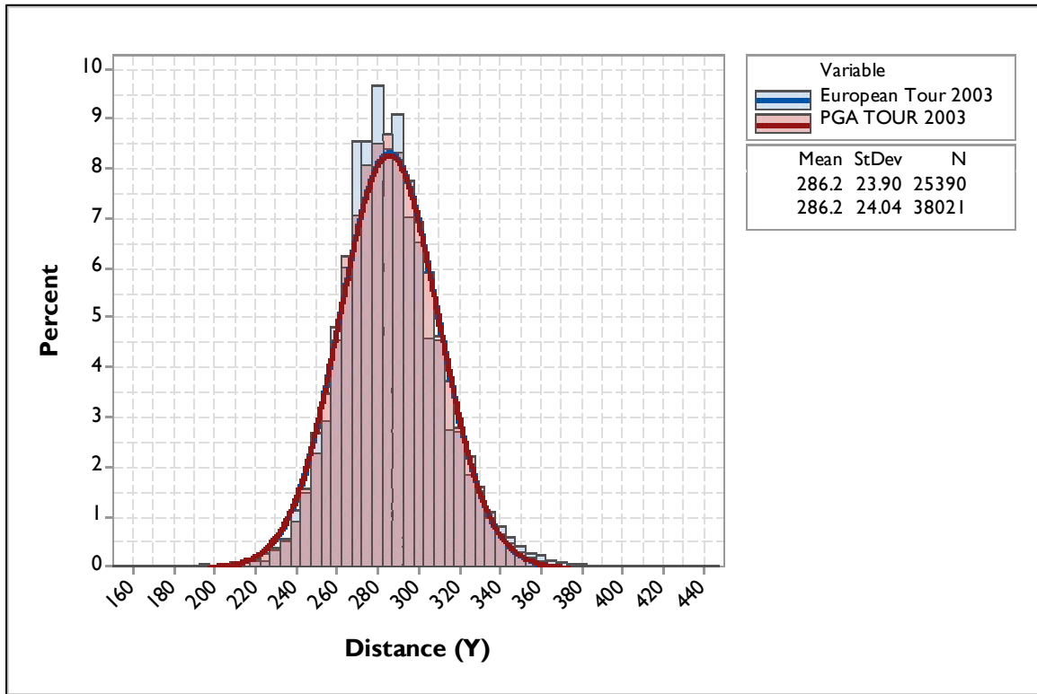
Figure 8. The distribution of distances on “measured” driving holes on the European and PGA TOUR in 2003.
