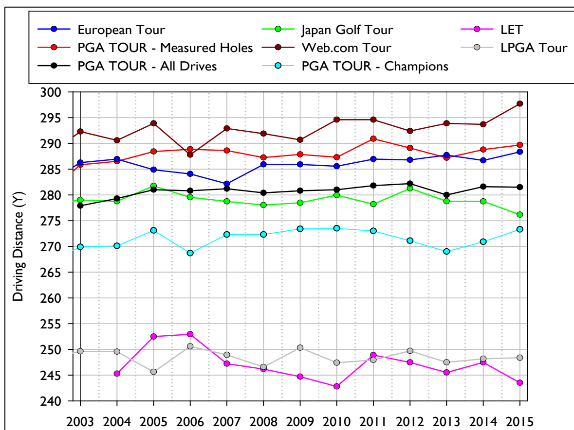
Figure 5. Average driving distance on the major tours since the first full season after the publication of the Joint Statement of Principles.
