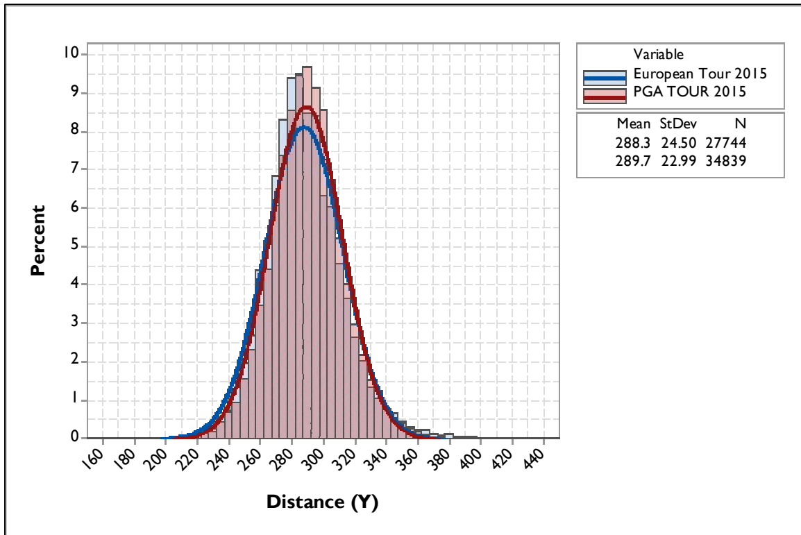
Figure 9. The distribution of distances of “measured” driving holes on the European and PGA TOUR in 2015.
